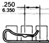
TO-126 CASE 7-290
