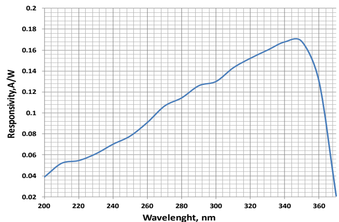
SPECTRAL RESPONSE
