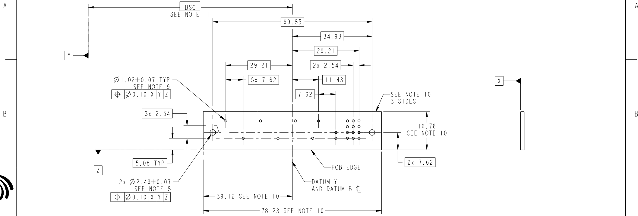
RECOMMENDED PCB LAYOUT
