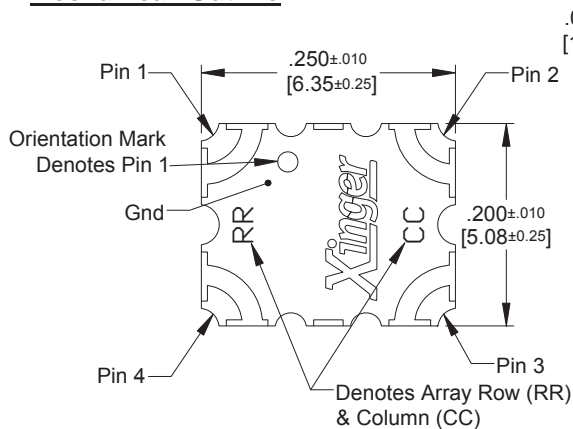
Dimensions are in Inches [Millimeters] XEC24P3-30G Mechanical Outline
