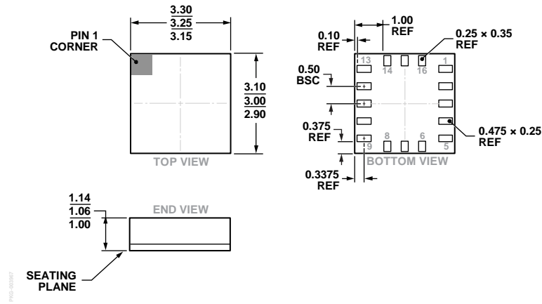
Figure 55. 16-Terminal Land Grid Array [LGA] (CC-16-4) Dimensions shown in millimeters
